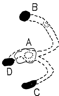
Fig. 14. A sketch of the relative positions of bright point II , outlined by the dashed curves and its brighter inner cores, outlined by the dotted curves, above the positive magnetic pole A (shaded in white), and the negative magnetic poles B , C , and D (shaded in black) in the photosphere.
